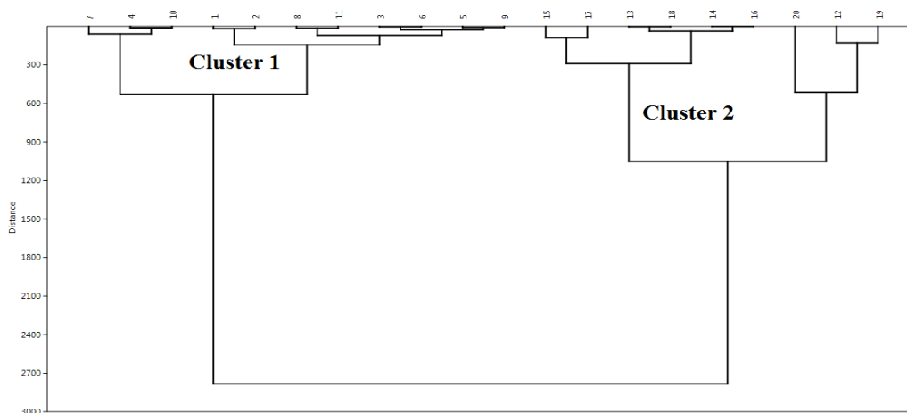
Fig.5.1 Dendrogram of Surface water trace elements
