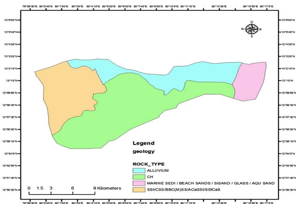
Fig 2. Geology map of the study area
